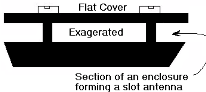
Figure 2 - "Natural" Slot Antenna
