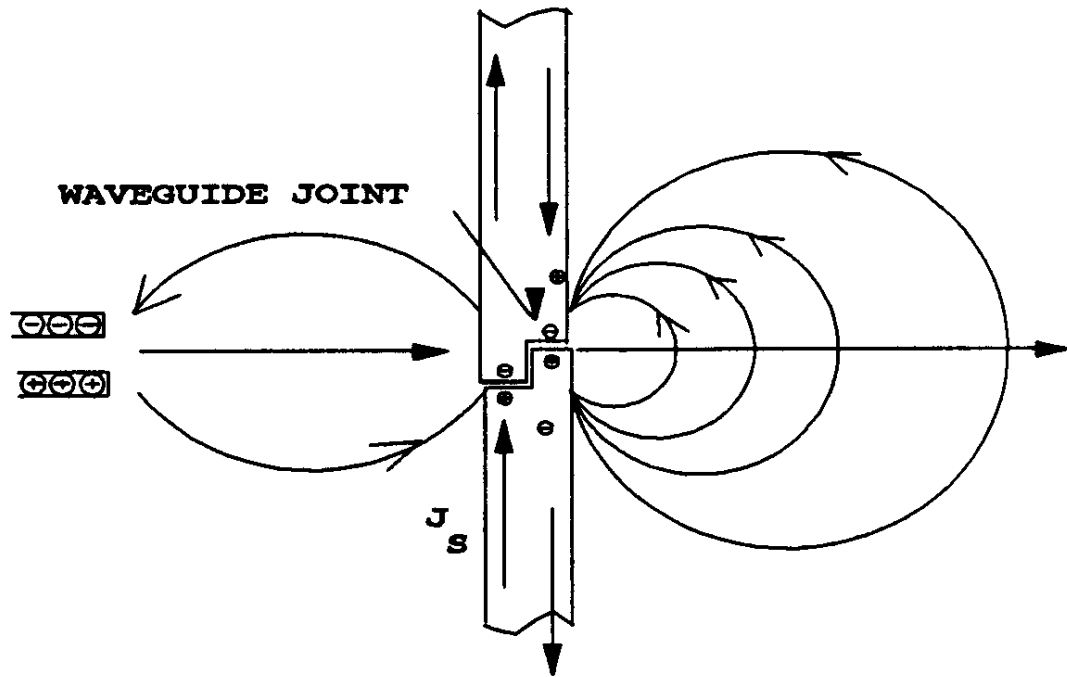
Figure 4 - Waveguide Condition Without Gasket
