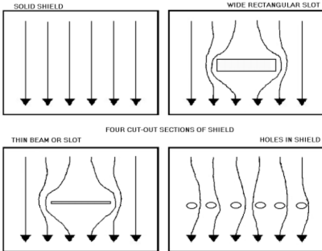
Figure 1 - How Shield Discontinuities Effect Current Flow
