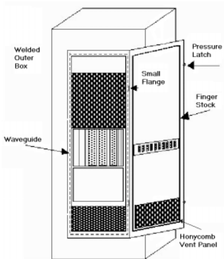
Figure 10 – High Attenuation Application of Fingerstock
