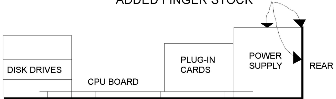
SIDE VIEW OF INTERNAL ASSEMBLY (DISK DRIVES AND POWER SUPPLY NOT TO SCALE)
