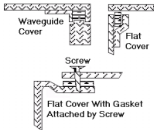
Figure 6 – Gasket Compression Bolting
