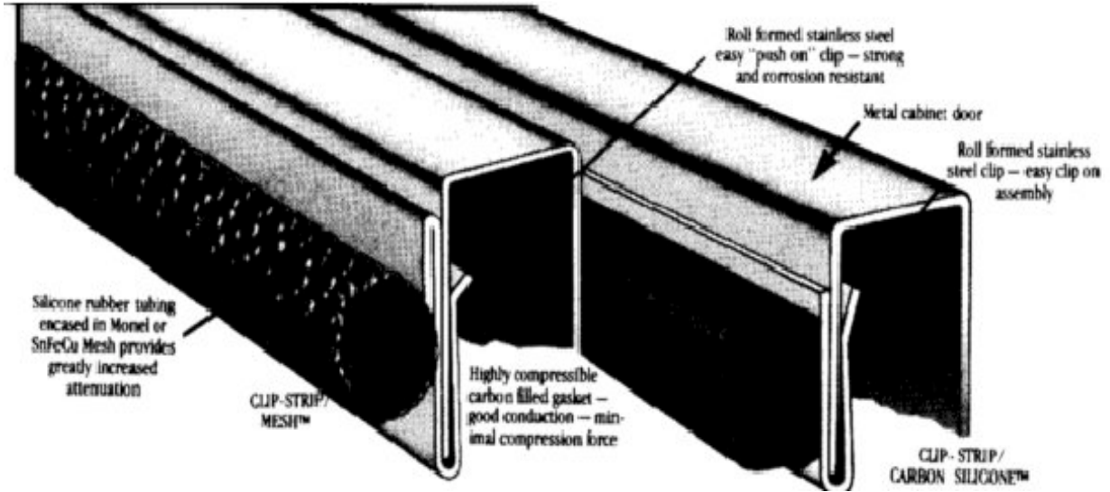
Figure 8 - Metal Braid Covered Foam Gasket
