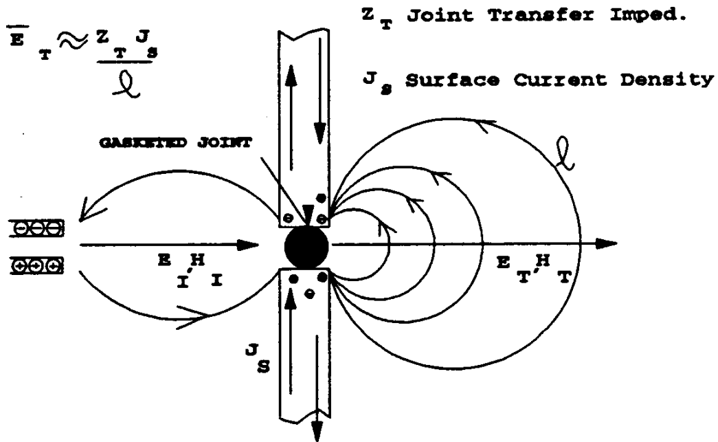
Figure 3 - Gasketed Joint Showing Less Abrupt Impedance
